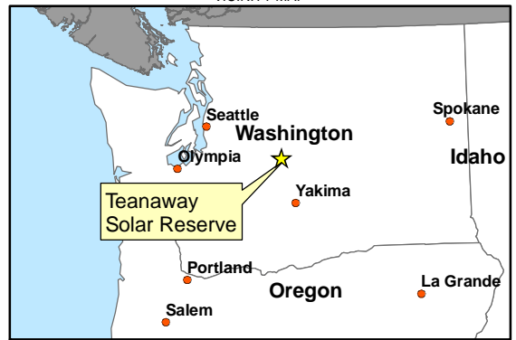
FIGURE 2 U.S. Geological Survey Topographic Map Teanaway Solar Reserve Kittitas County, Washington
